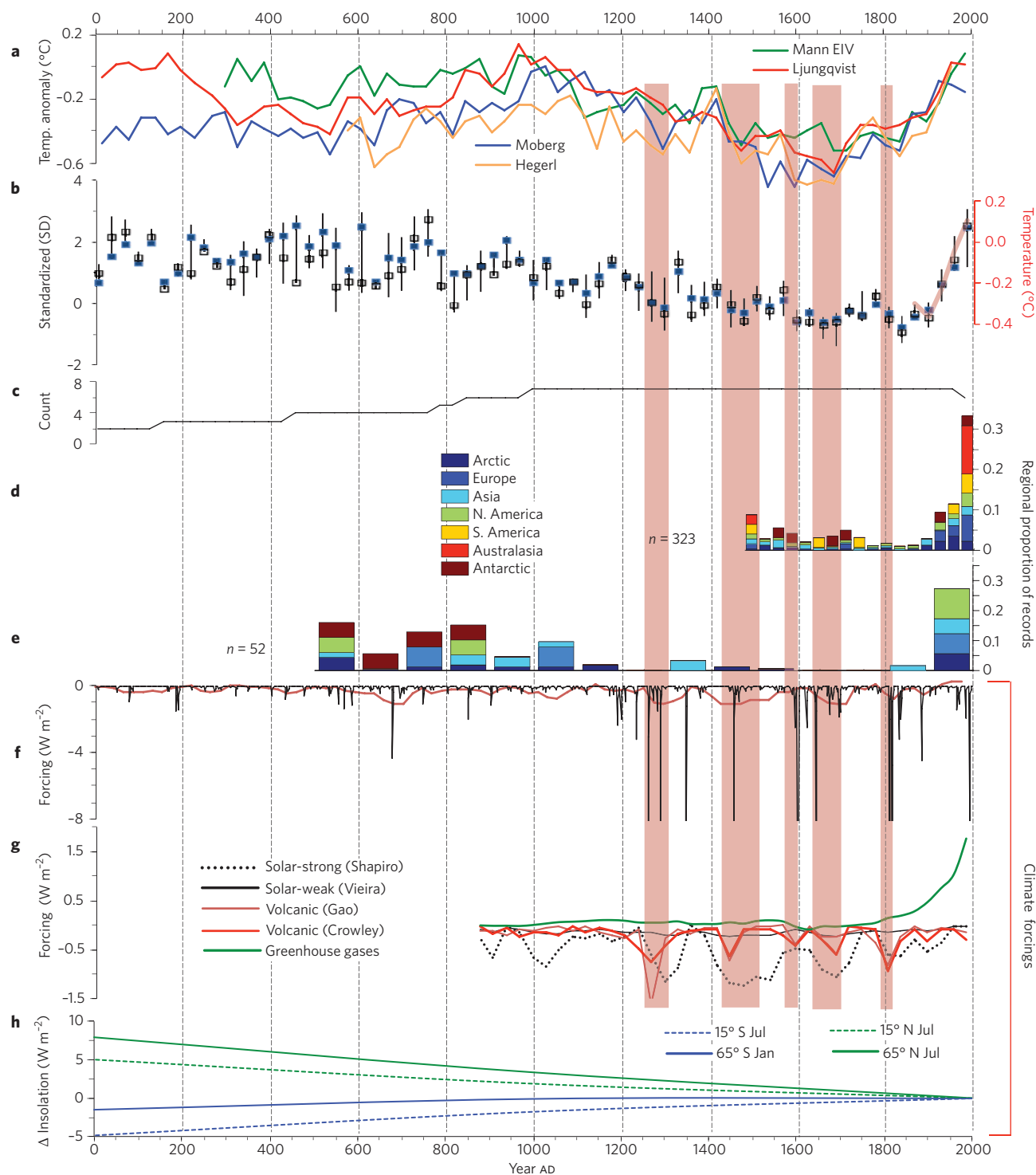
Figure 4 | Composite temperature reconstructions with climate forcings and previous hemisphere-scale reconstructions. a , Previously published Northern Hemisphere 30-year-mean temperature reconstructions relative to the 1961–1990 reference period 45,43–54 . b , Standardized 30-year-mean temperatures averaged across all seven continental-scale regions. Blue symbols are area-weighted averages using domain areas listed in Table 1, and bars show twenty-fifth and seventy-fifth unweighted percentiles to illustrate the variability among regions; open black boxes are unweighted medians. The red line is the 30-year-average annual global temperature from the HadCRUT4 (ref. 29) instrumental time series relative to 1961–1990, and scaled visually to match the standardized values over the instrumental period. c , Running count of the number of regional reconstructions. d , For each 30-year period since AD 1500, the proportion of individual proxy records within each region that indicate the highest temperature during that 30-year period. e , For each century since AD 500, the proportion of individual proxy records within each region that indicate the highest temperature during that century. f , Long-term volcanic forcing from ref. 16 (black curve; spikes beyond -8 \text{ W m}^{-2} are truncated), and solar forcing from ref. 17 (red curve). g , Radiative forcings relative to AD 2000 smoothed using 30-year averages from ref. 31, including: two estimates of volcanic forcing 46,47 ; two estimates of solar forcing that span the range from strong 48 to weak 49 ; and well-mixed greenhouse gases relative to AD 850. h , Change in summer (July and January) insolation at 65° N/S and 15° N/S latitudes relative to AD 2000 from ref. 50. Vertical red bands indicate volcanic-solar downturns as defined in Methods.
